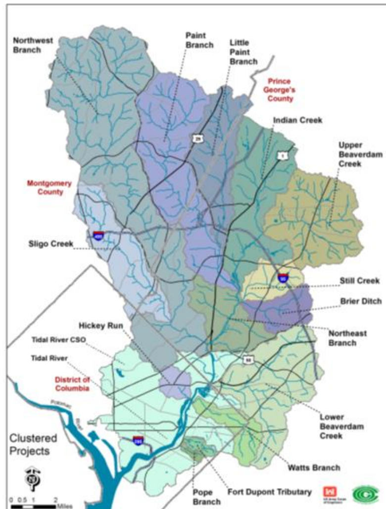
Anacostia Watershed and its Subwatersheds
