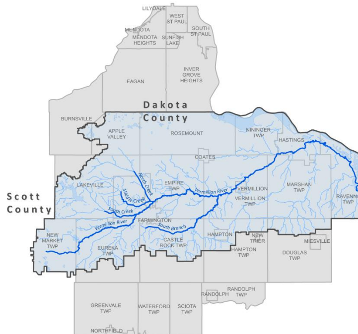
Vermillion River Watershed Map
