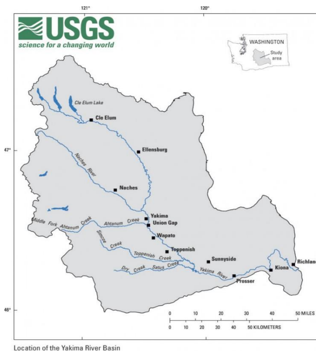
Location of the Yakima River Basin
