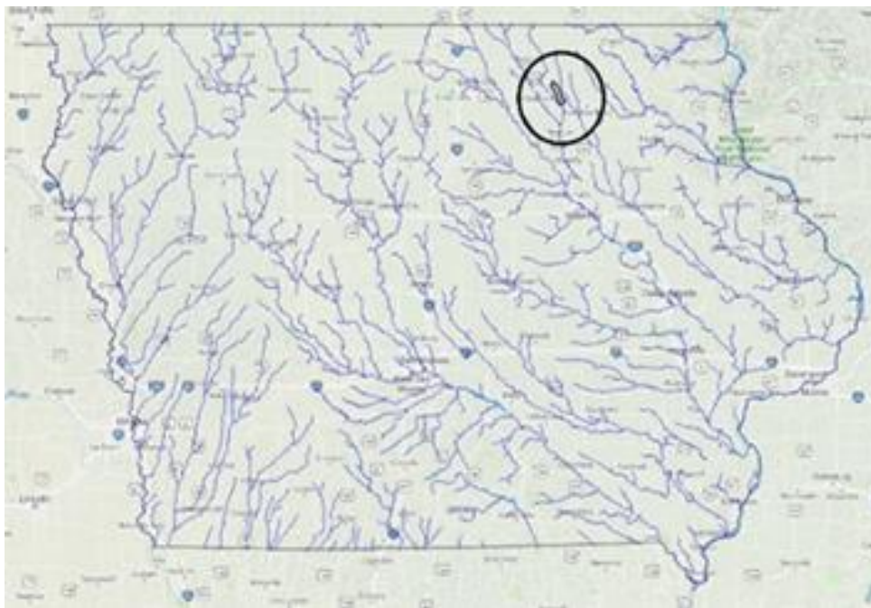
Figure 1: Location of the Beaver Creek Watershed
