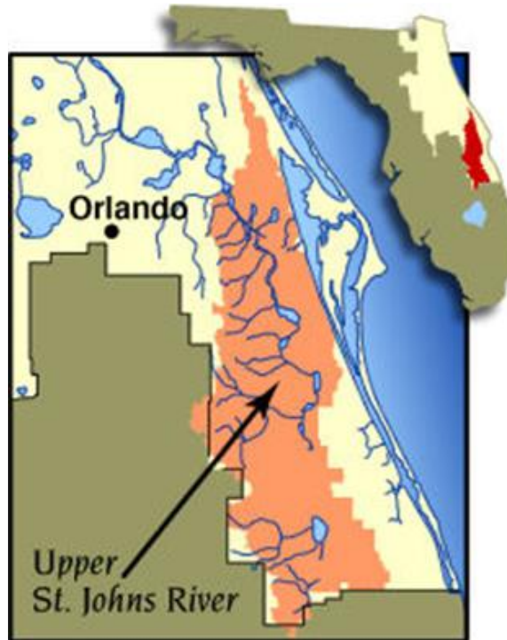
Location of the Upper St. Johns River Basin In the state of Florida Map credit: SJRWMD
