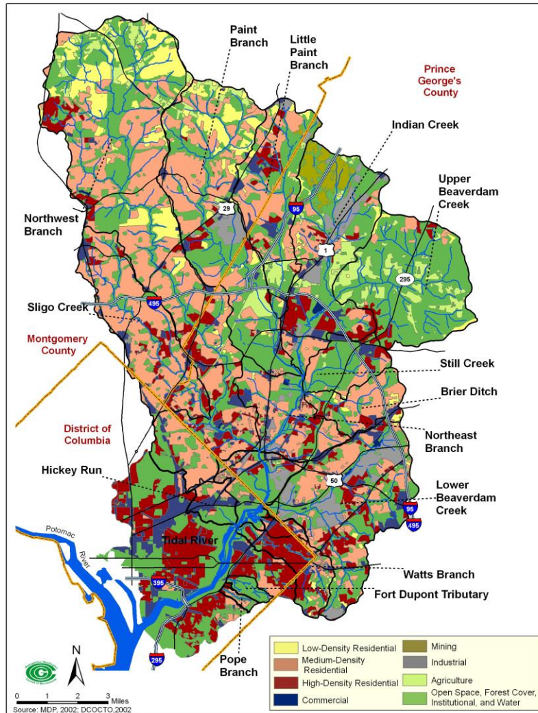
Land use within the Anacostia Watershed
