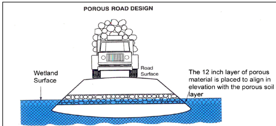
Figure 8. Porous Road Design Using Large Stone. (Re-printed courtesy of the United States Forest Service)
