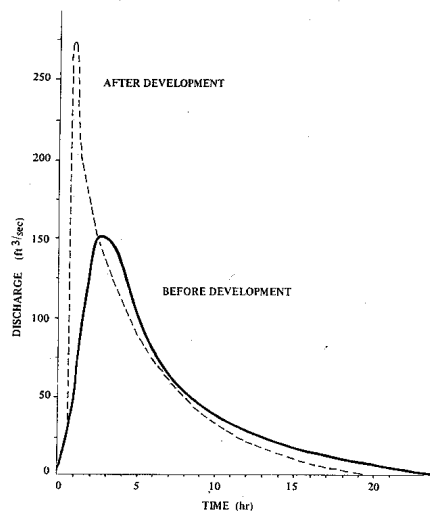
Figure 28. Urban development increases peak discharge in rivers. Comparisons of hydrographs for a watershed before and after development (redrawn from Fusillo 1981).
