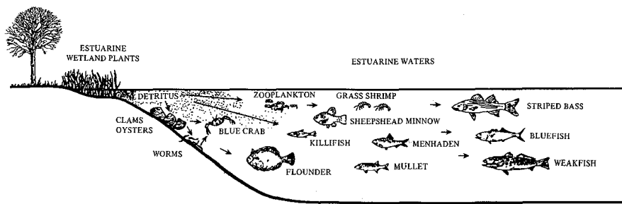
Figure 26. Simplified food pathways from estuarine wetland vegetation to commercially and recreationally important fishes and shellfishes.
