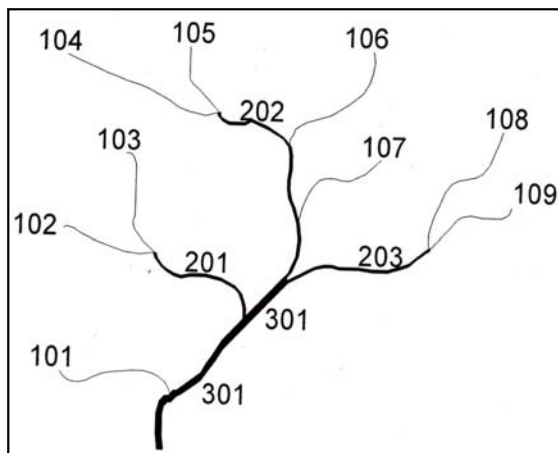
Figure 12: Strahler's Stream Order Diagram
