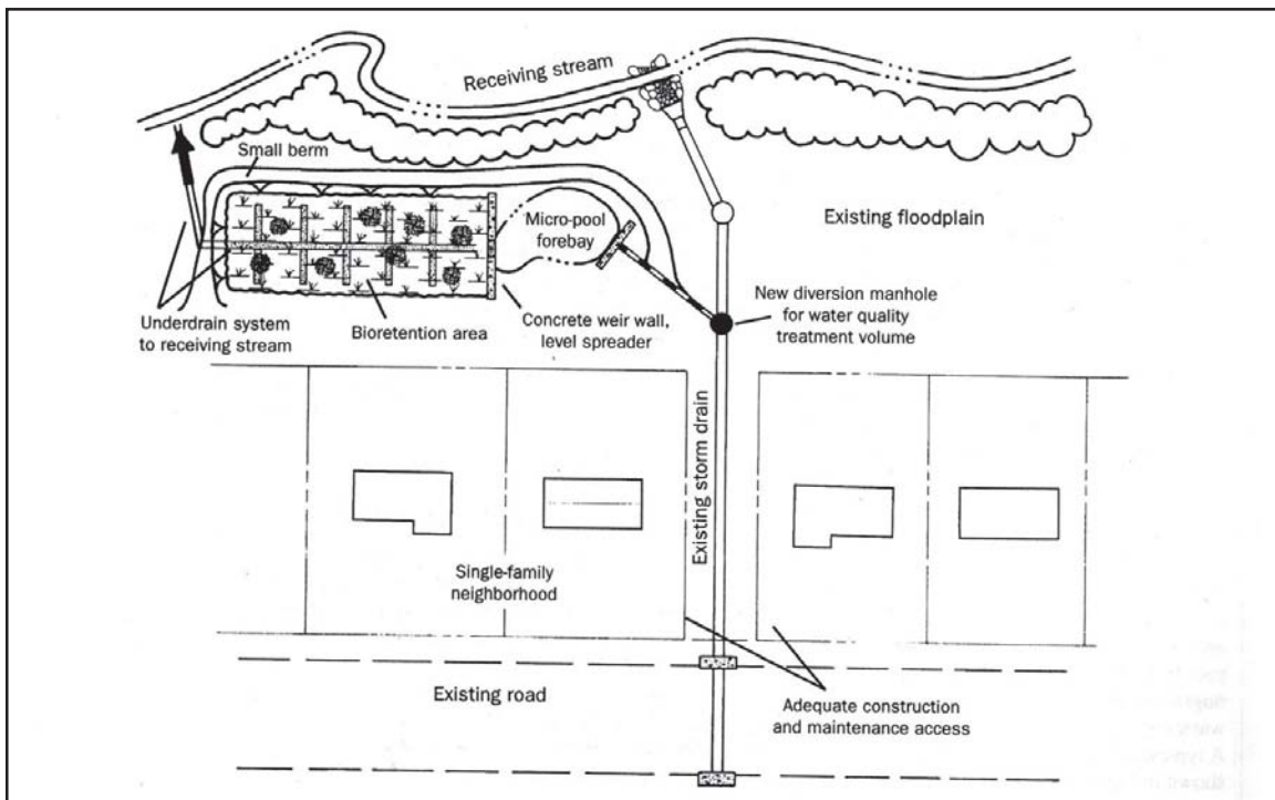
Figure 17: Schematic of Off-line Retrofit in the Riparian Corridor
