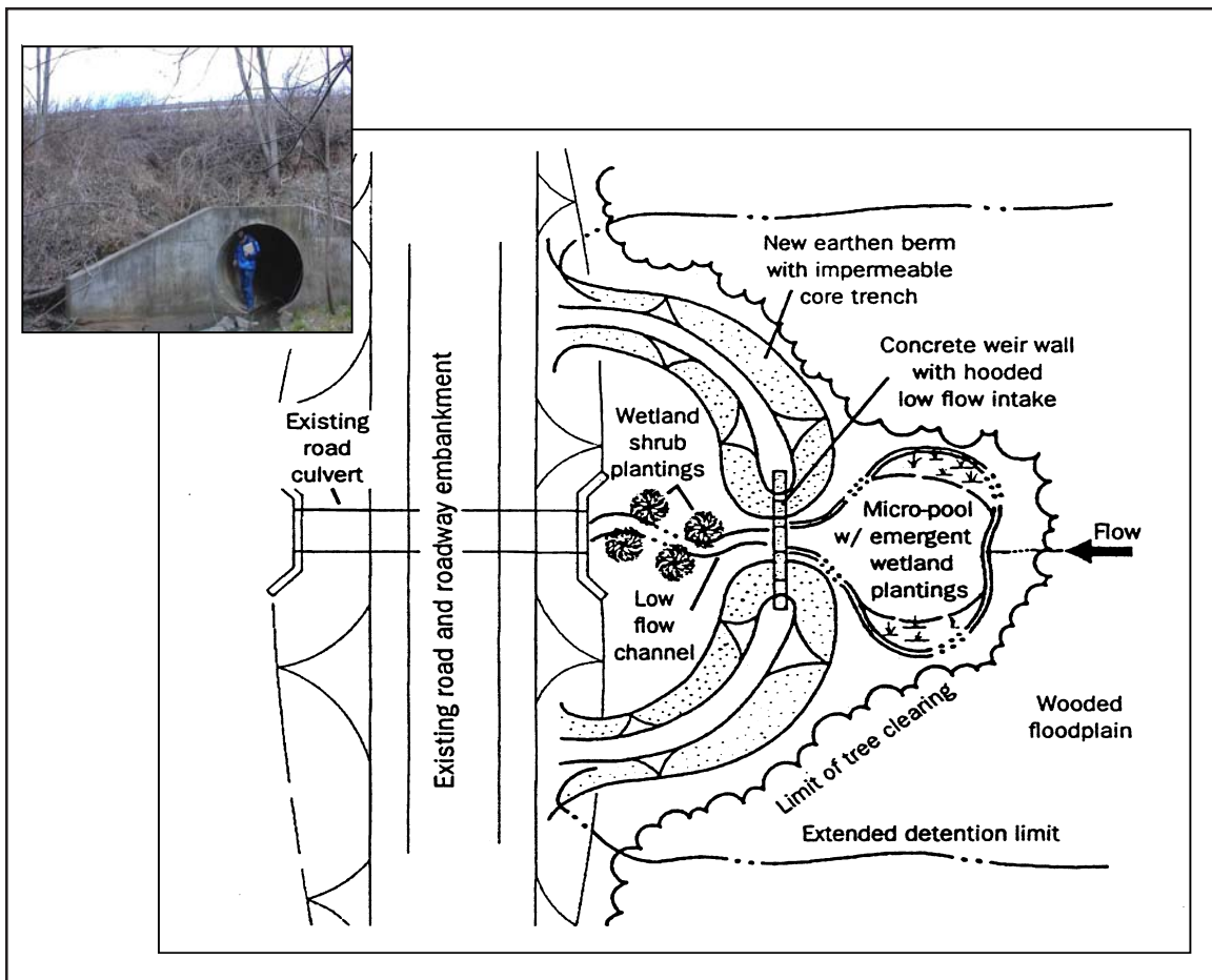
Figure 36: Schematic of Upstream Storage Retrofit
