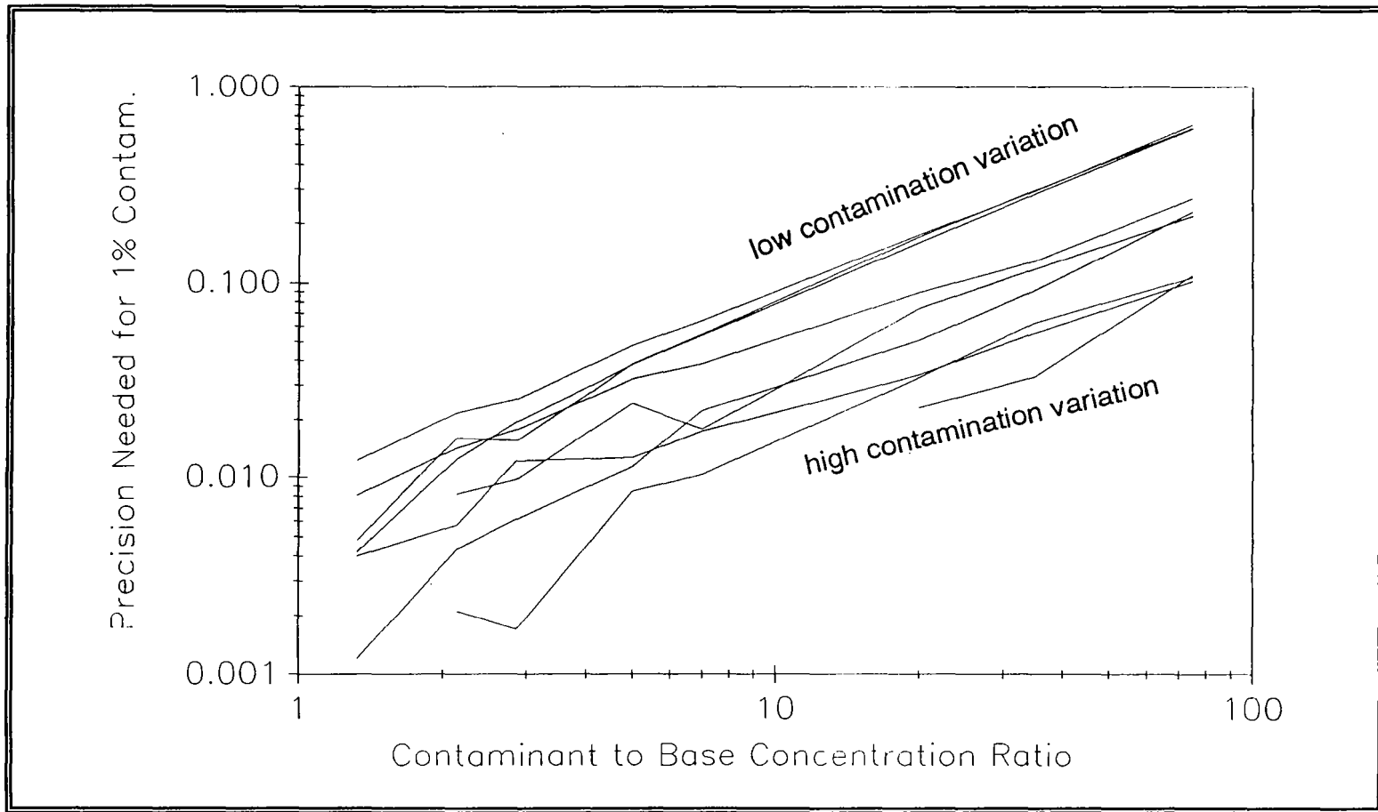
Figure 8. Analysis precision needed for detection of one percent contamination at ninety percent confidence.
