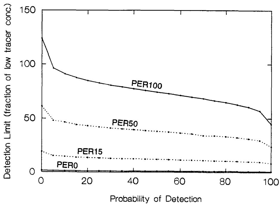
Figure 7. Required detection limits for low COV mixture components having means differing by 75 times.
