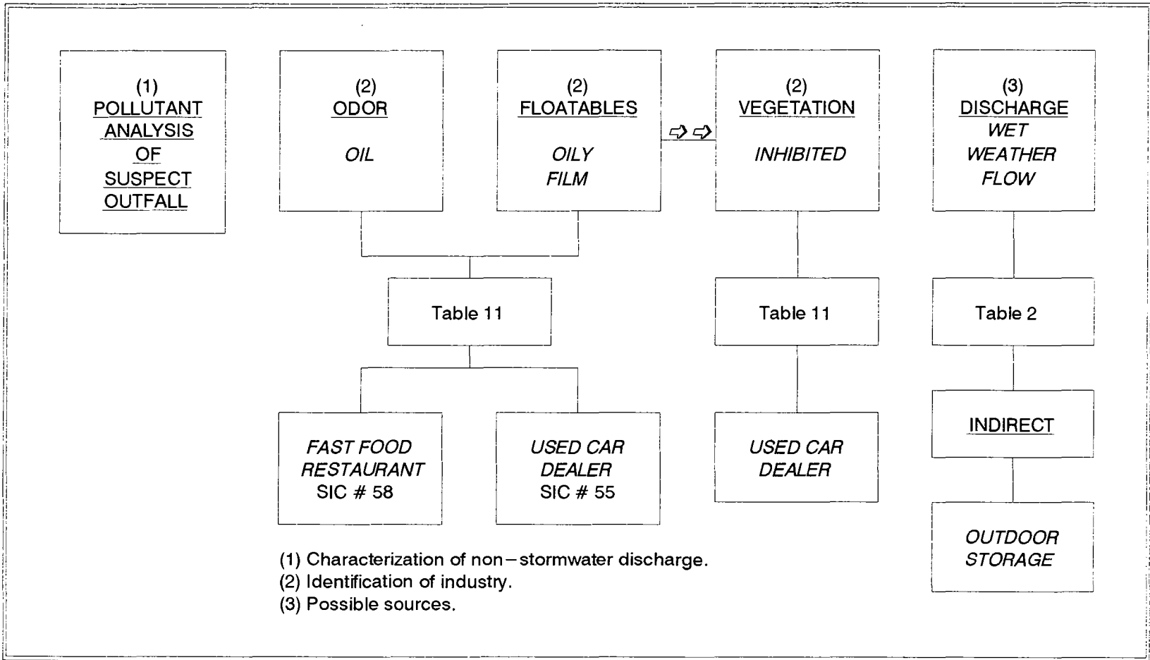
Figure 14. Flowsheet for Industrial Case Example 3.
