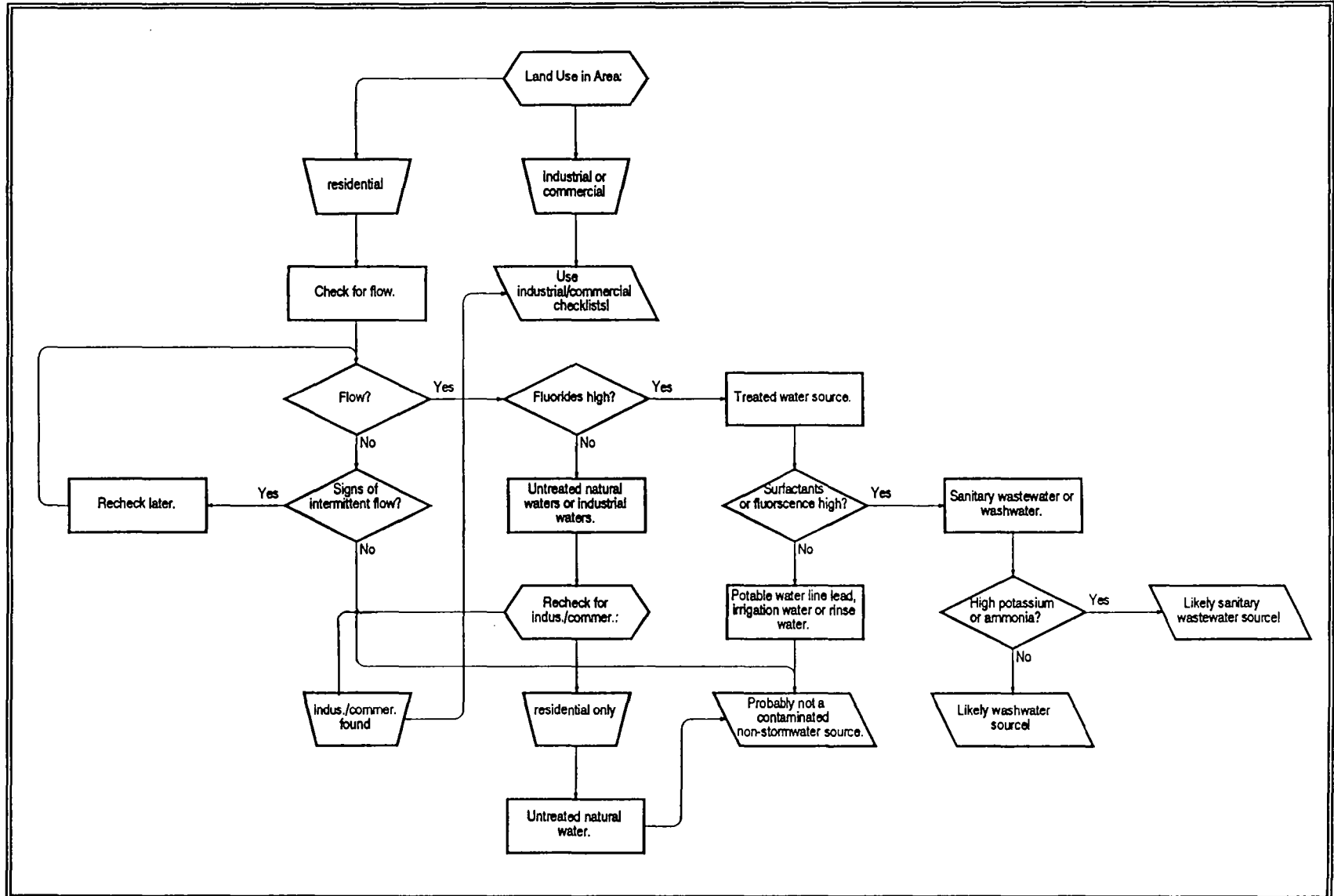
Figure 10. Flow chart to identify residential area non-stormwater flow sources.
