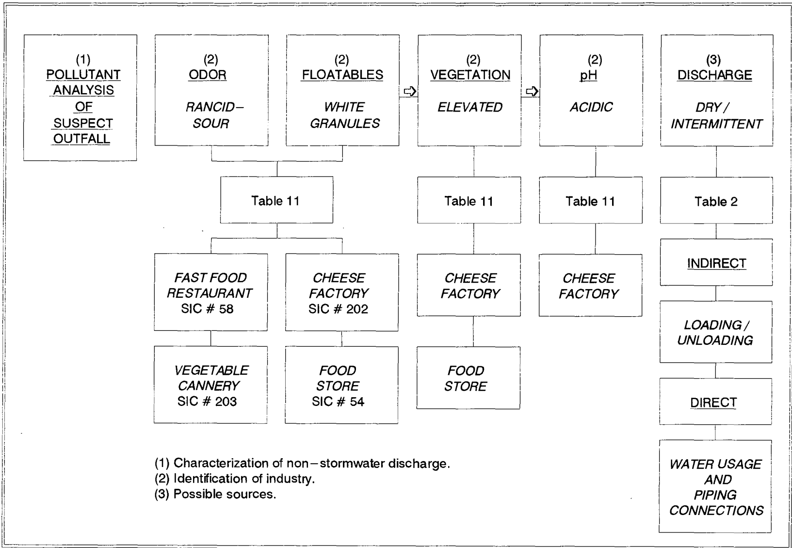
Figure 13. Flowsheet for Industrial Case Example 2.
