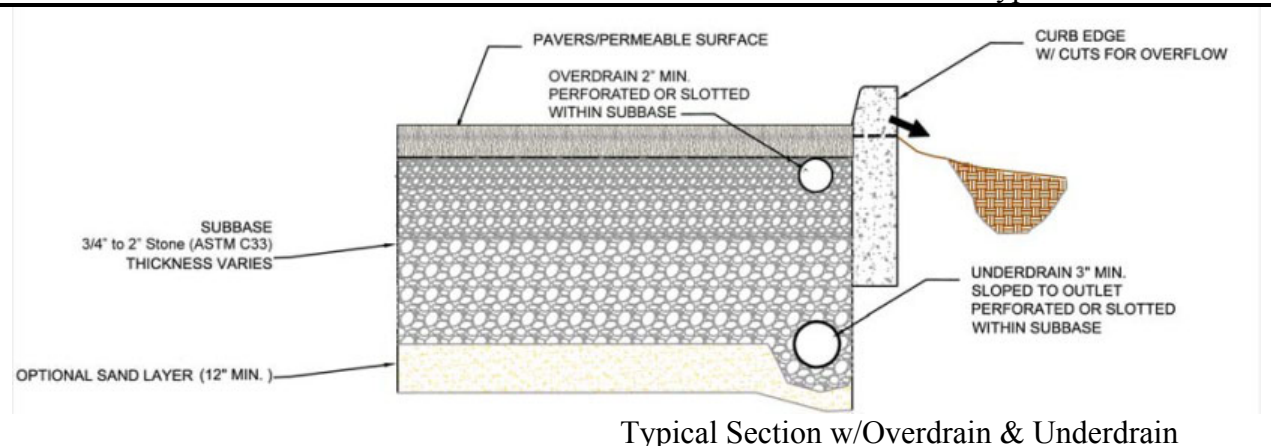
Typical Section
