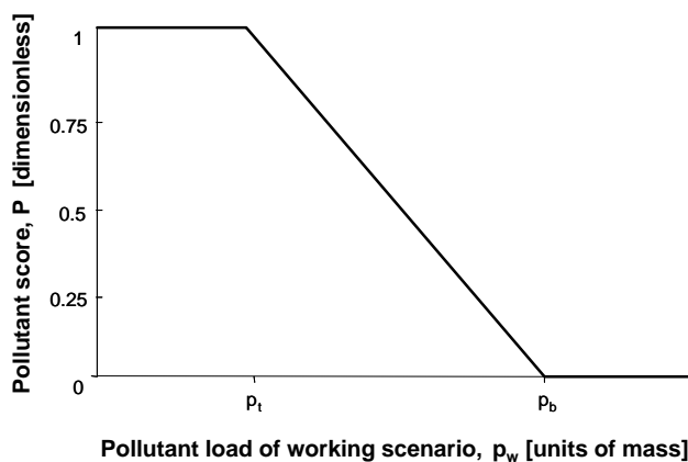
Figure 2. Pollutant score fitness function.
