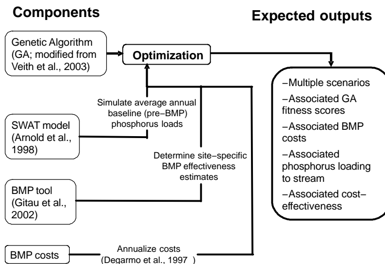
Figure 1. Flowchart of optimization methodology showing components and their interactions.
