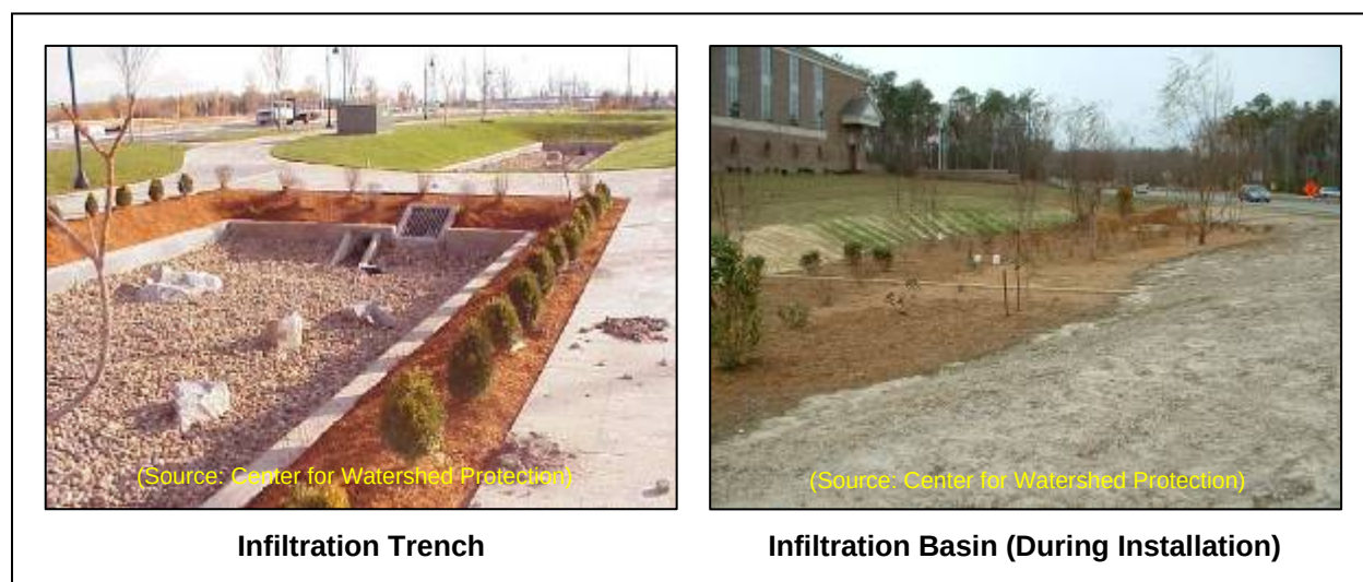
Figure 7.45: Infiltration Practices
