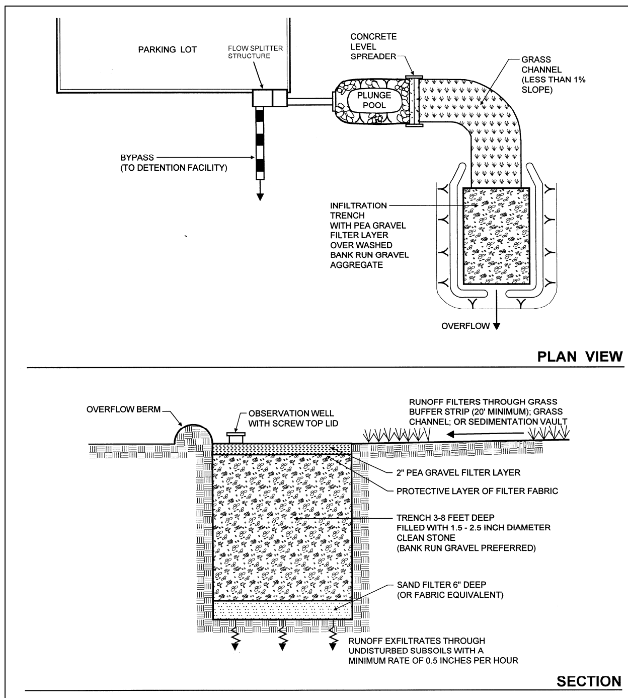
Figure 8.26: Schematic of a Typical Infiltration Trench
