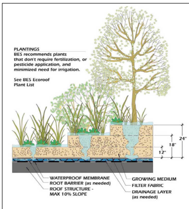
Figure 7.26: Intensive Green Roof System
