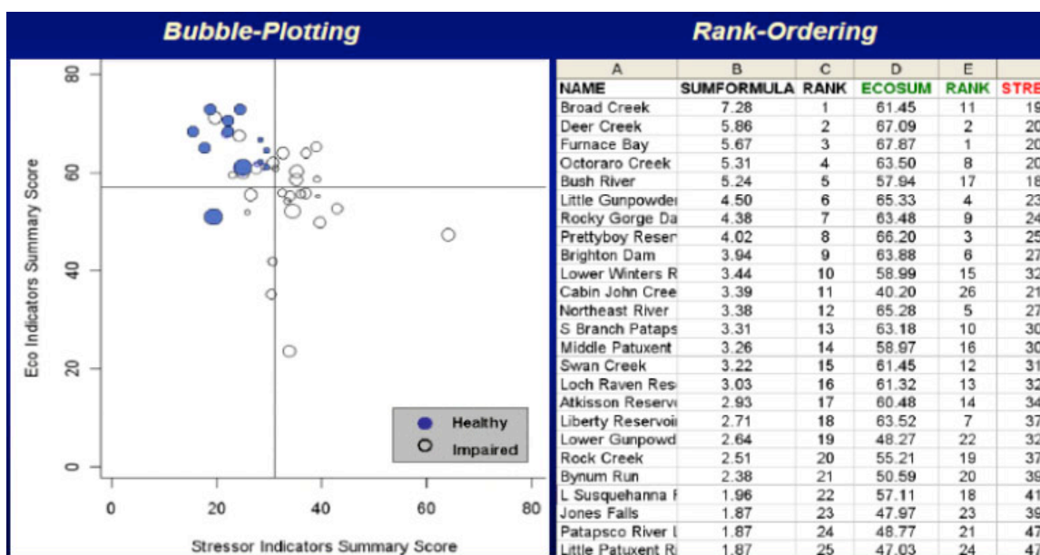
Figure 38: Bubble plots and rank-ordered scores for ecological, stressor, and social context indicators for each HUC-12 watershed generated by EPA RPS. Stanley, S., S. Grigsby, T. Hraby, and P. Olson. 2009. Puget Sound Watershed Characterization Project: Description of Methods, Models and Analysis. Washington State Department of Ecology. Publication #10-06-005. Olympia, WA.
