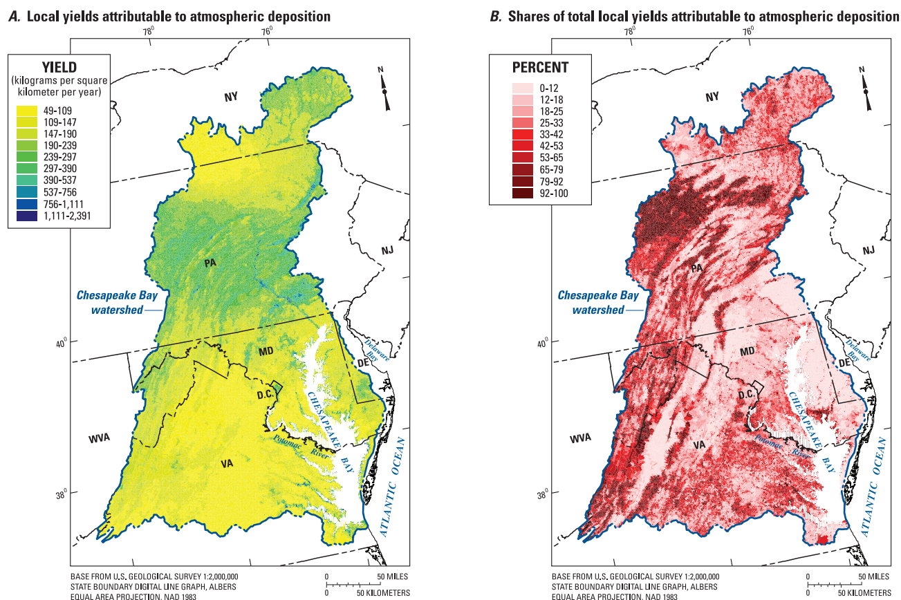
Figure 7. Estimated local (A) yields and (B) source shares of total nitrogen from atmospheric deposition.
