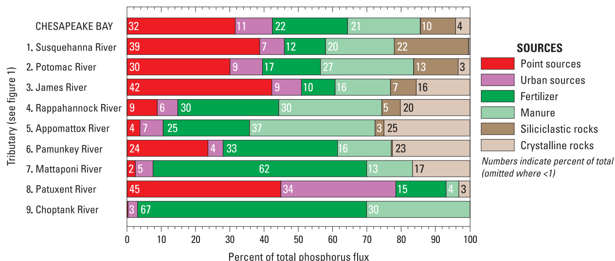
Figure 12. Estimated shares of total phosphorus contributions from various watershed sources to Chesapeake Bay and to major tributaries at selected monitoring stations.
