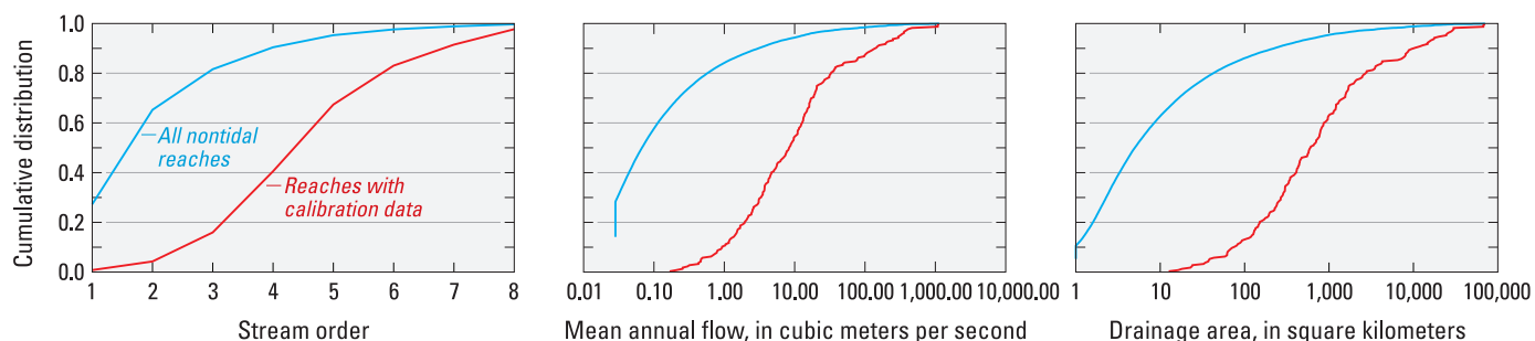
Figure 4. The distribution of stream order, streamflow, and watershed size among modeled stream reaches in the Chesapeake Bay watershed, and those with calibration stations.
