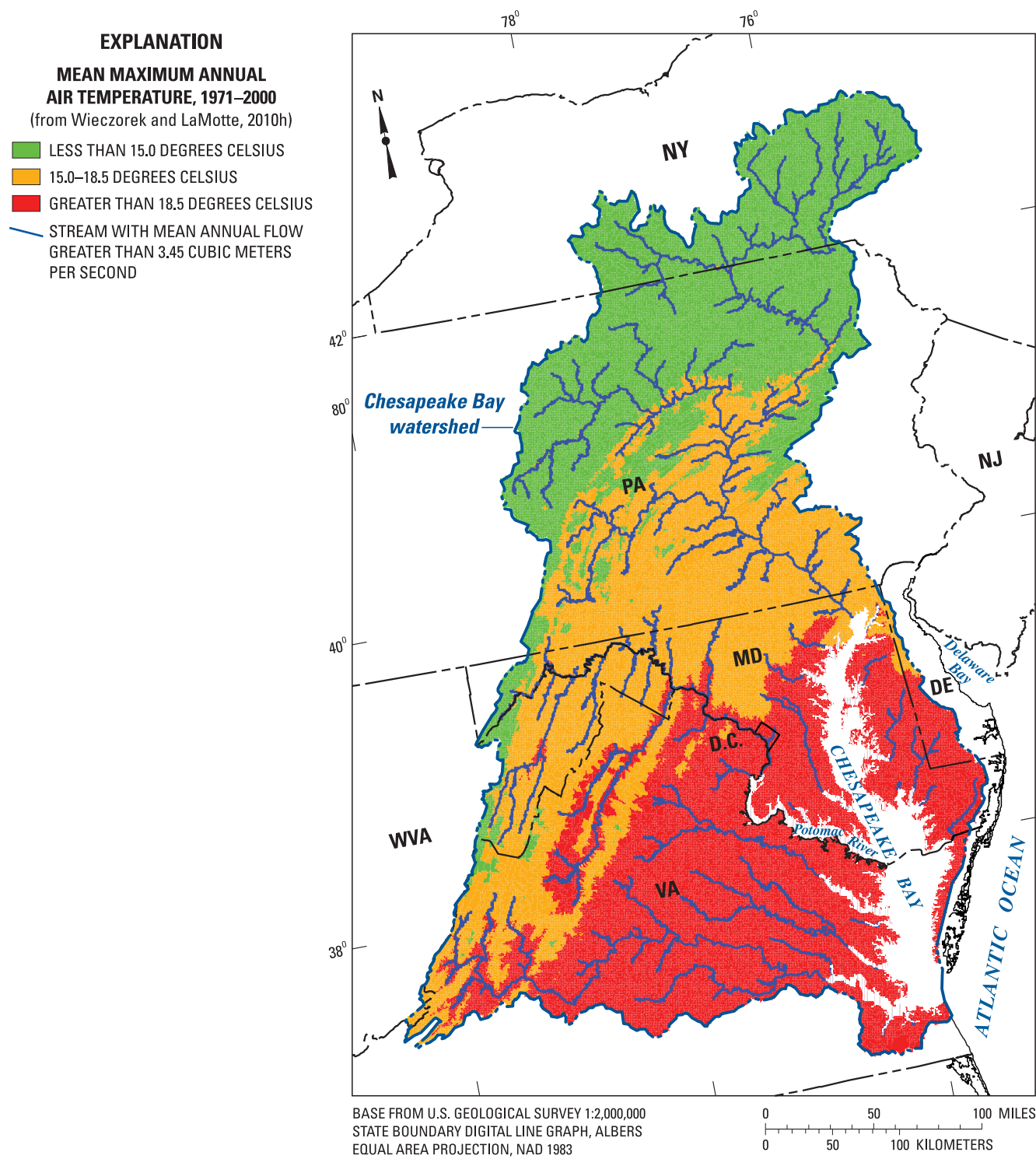
Figure 5. Mean annual maximum air temperature, 1971–2000, and streams with mean annual flow greater than 3.45 cubic meters per second.
