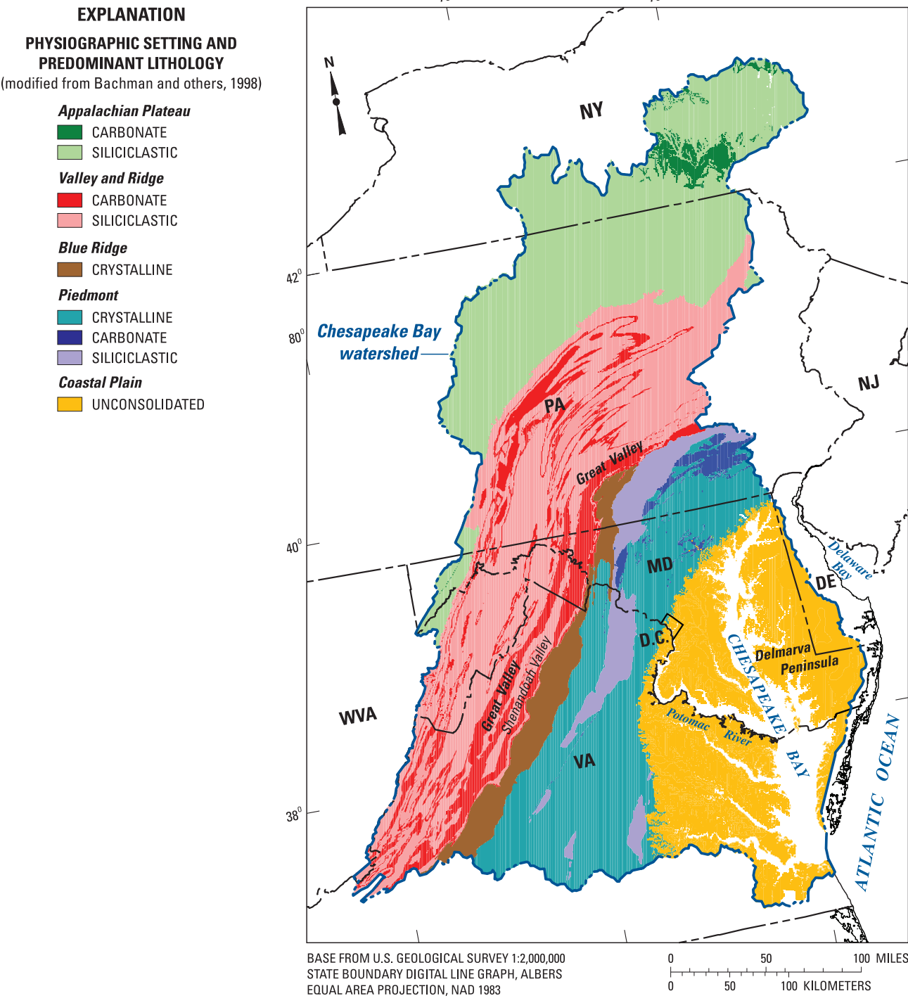
Figure 2. Hydrogeologic settings within the Chesapeake Bay watershed.
