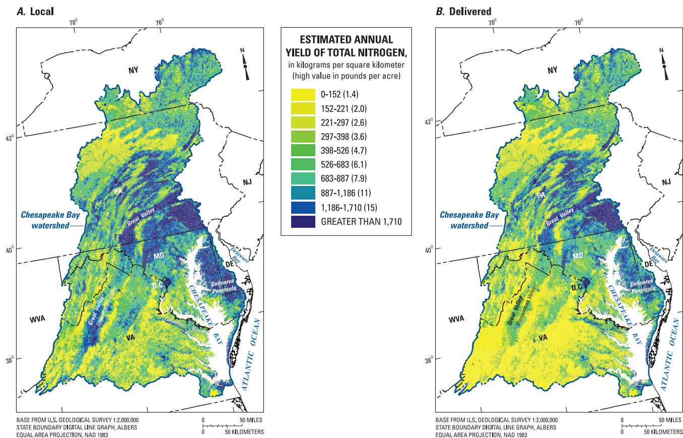
Figure 9. Estimated (A) local and (B) delivered yields of total nitrogen (TN). Local yields represent TN flux delivered to streams from individual local catchments; delivered yields represent TN flux delivered to downstream terminal reaches (generally tidal waters).
