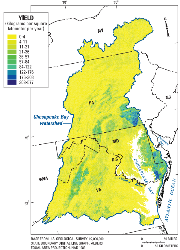
D. Total phosphorus attributable to manure
