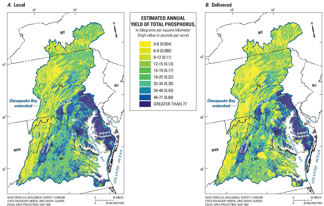
Figure 10. Estimated (A) local and (B) delivered yields of total phosphorus (TP). Local yields represent TP flux delivered to streams from individual local catchments; delivered yields represent TP flux delivered to downstream terminal reaches (generally tidal waters).
