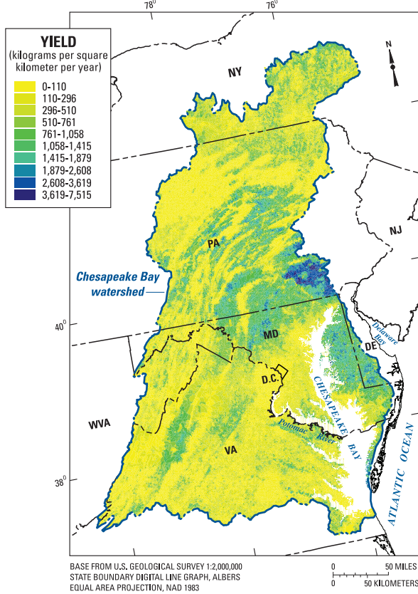
C. Total phosphorus attributable to fertilizer application
