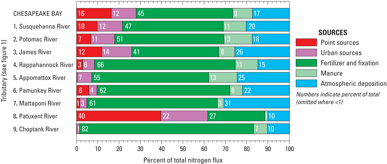
Figure 11. Estimated shares of total nitrogen contributions from various watershed sources to Chesapeake Bay and to major tributaries at selected monitoring stations.
