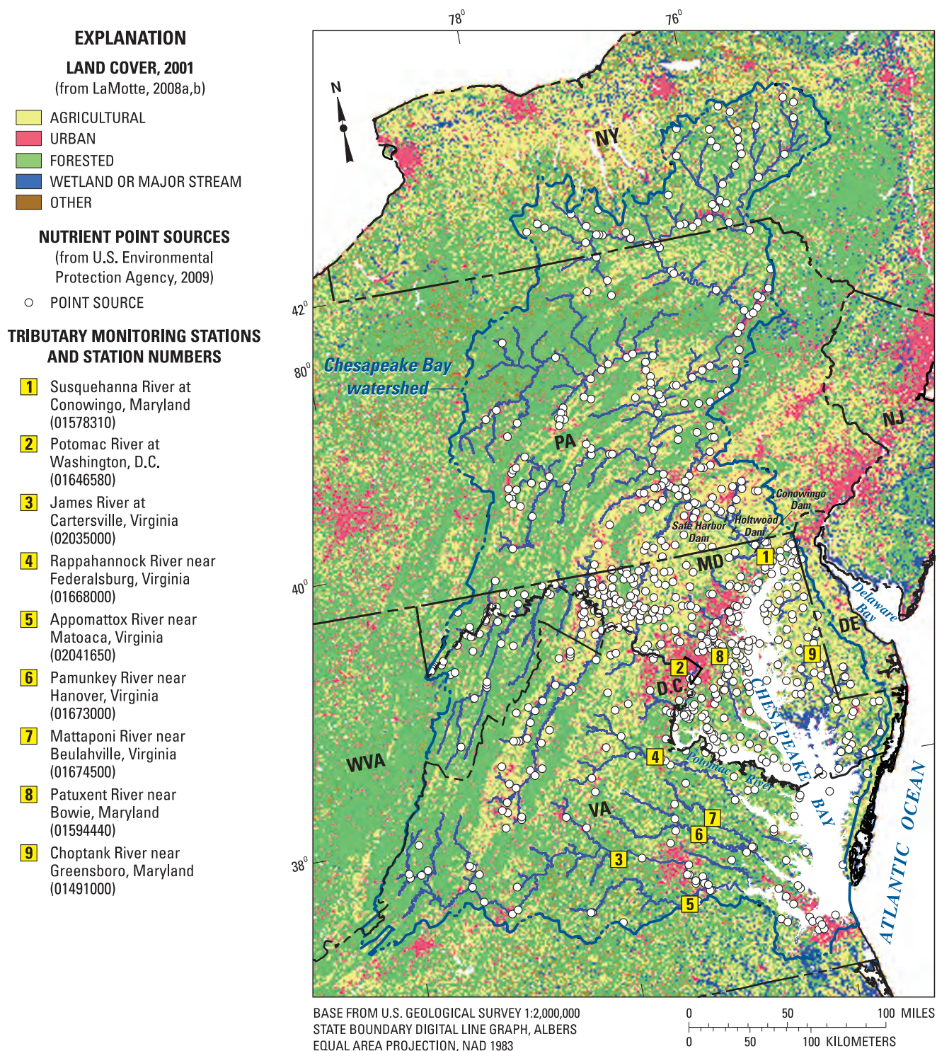
Figure 1. Location of the Chesapeake Bay watershed and vicinity, including generalized land cover, point sources, and selected long-term stream monitoring stations for nutrient flux.
