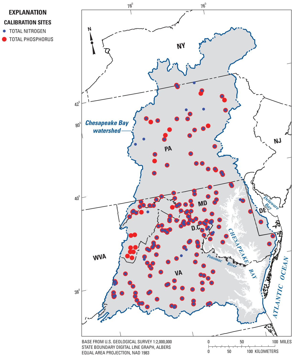
Figure 3. Location of stations for which mean annual flux estimates of total nitrogen and (or) total phosphorus were computed for use in SPARROW model calibration.
