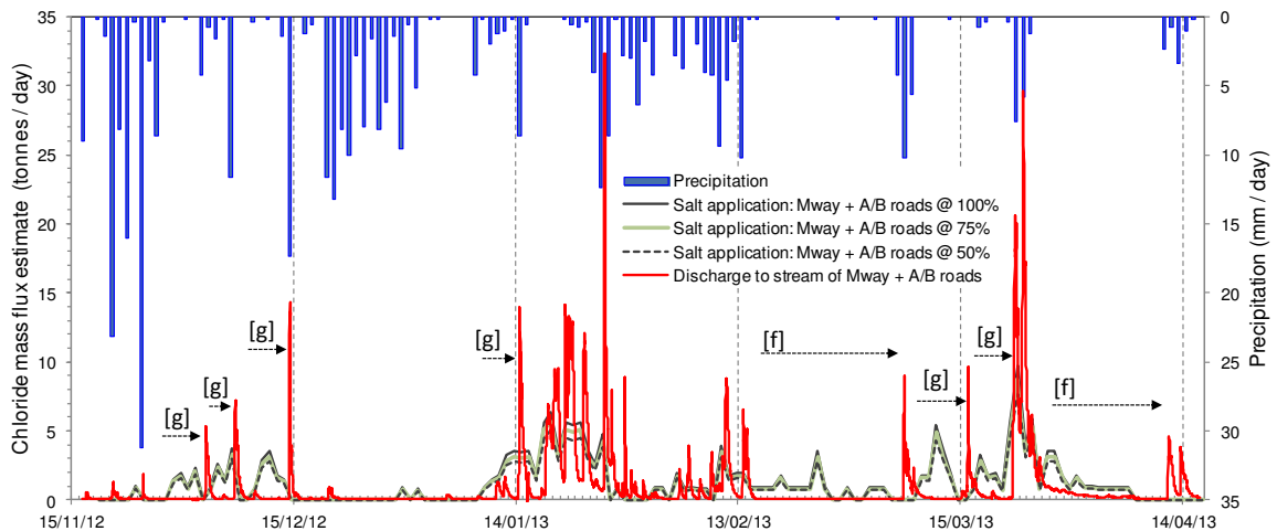
Fig. 9. Winter 2012-13 chloride mass flux comparison of highway runoff discharge to stream (estimated from Eq. (3) and observed stream data) with various highway salt application estimates and daily precipitation data. Labels [f] and [g] are discussed in the text.
