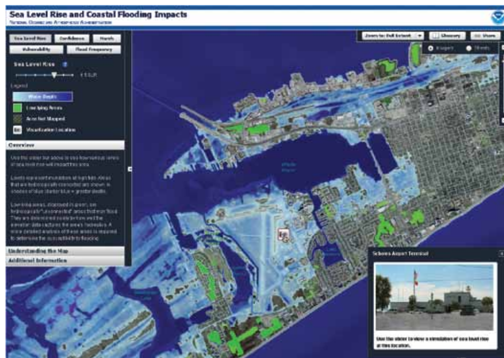
Figure 6: Sea Level Rise and Coastal Flooding Impacts Viewer for Galveston, Texas. Use the tool by going to www.csc.noaa.gov/SLR .
