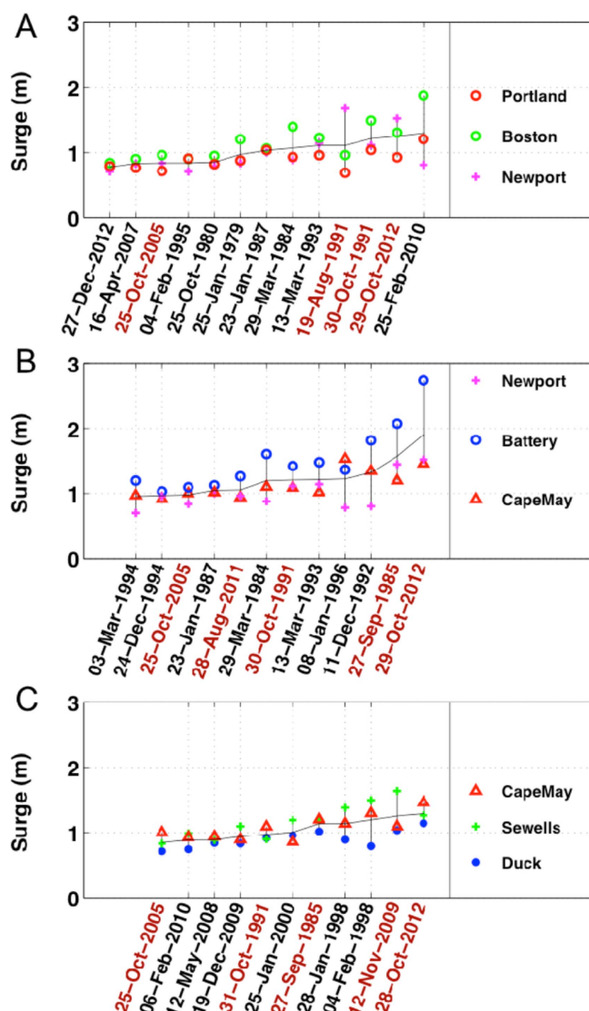
Figure 3. Surge values and dates for the storms that caused surge to exceed the 1-year RL at three consecutive stations, ranked largest to smallest from right to left, based on the multi-site average of the surge amplitudes. Panel (a) shows results for Portland, ME—Boston, MA—Newport, RI; (b) shows Newport, RI—The Battery, NY—Cape May, NJ; (c) shows Cape May, NJ—Sewells Point, VA—Duck, NC. Color-coding of dates indicates storm association: hurricanes (red) and ETCs (black). The thin black line indicates the multi-station mean value for each event.
