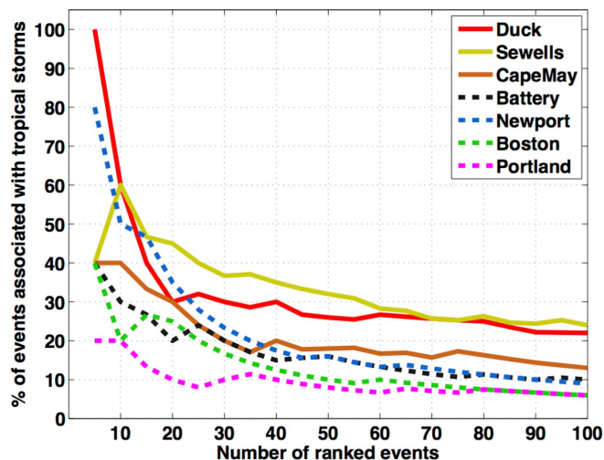
Figure 2. Percentage of surge events that are caused by hurricanes versus number of ranked events considered, per station. The solid lines indicate stations in this study located south of New York City. The dashed lines indicate those north of New York City. The percentages are calculated starting with the top 5 events at an interval of 5, up to the top 100.
